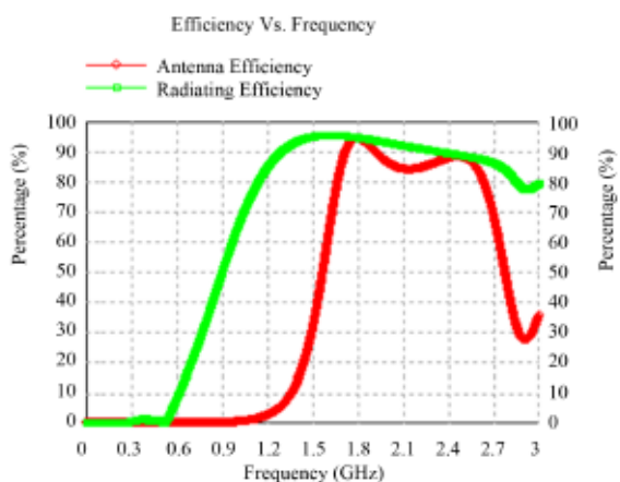
Figure 7. Efficiency Plot of the Microstrip Patch Antenna.
