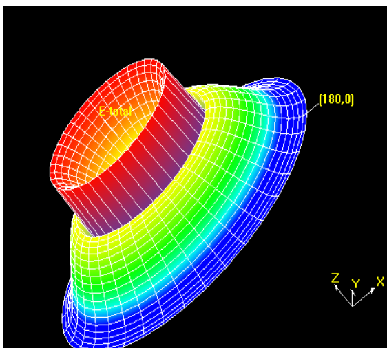
Figure 5. 3D Radiation Pattern Plot of the Microstrip Patch.
