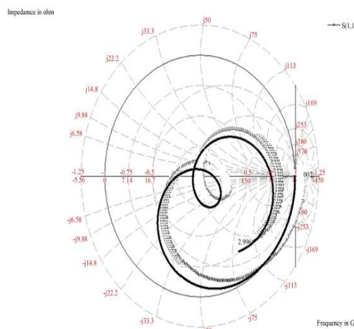
Figure 4. Smith chart of the microstrip patch antenna.
