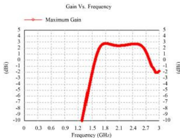
Figure 8. Maximum Gain Plot of Microstrip Patch Antenna.
